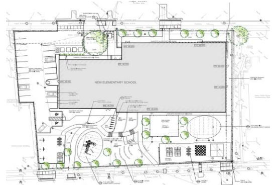
Site Plan
