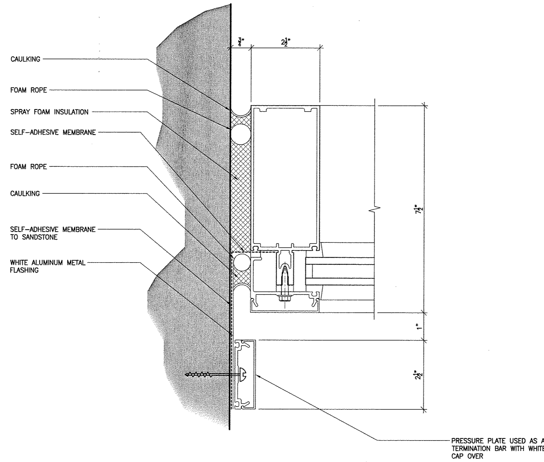
2 DETAIL - TUBE MULLION WITH PERIMTER PRESSURE PLATE 0 .5 1 2 4
