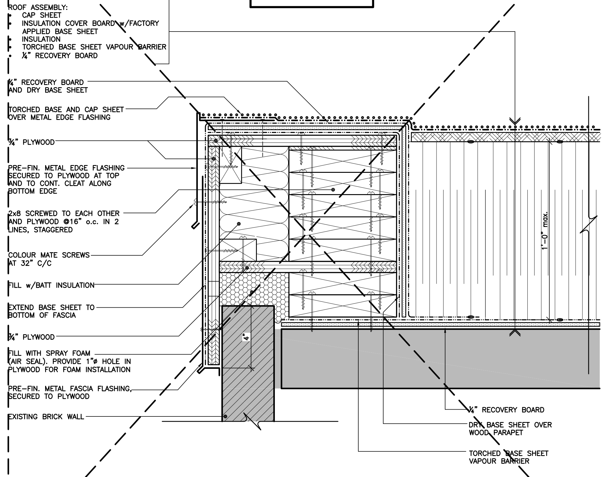
SECTION DETAIL ROOF EDGE AT ROOF C
