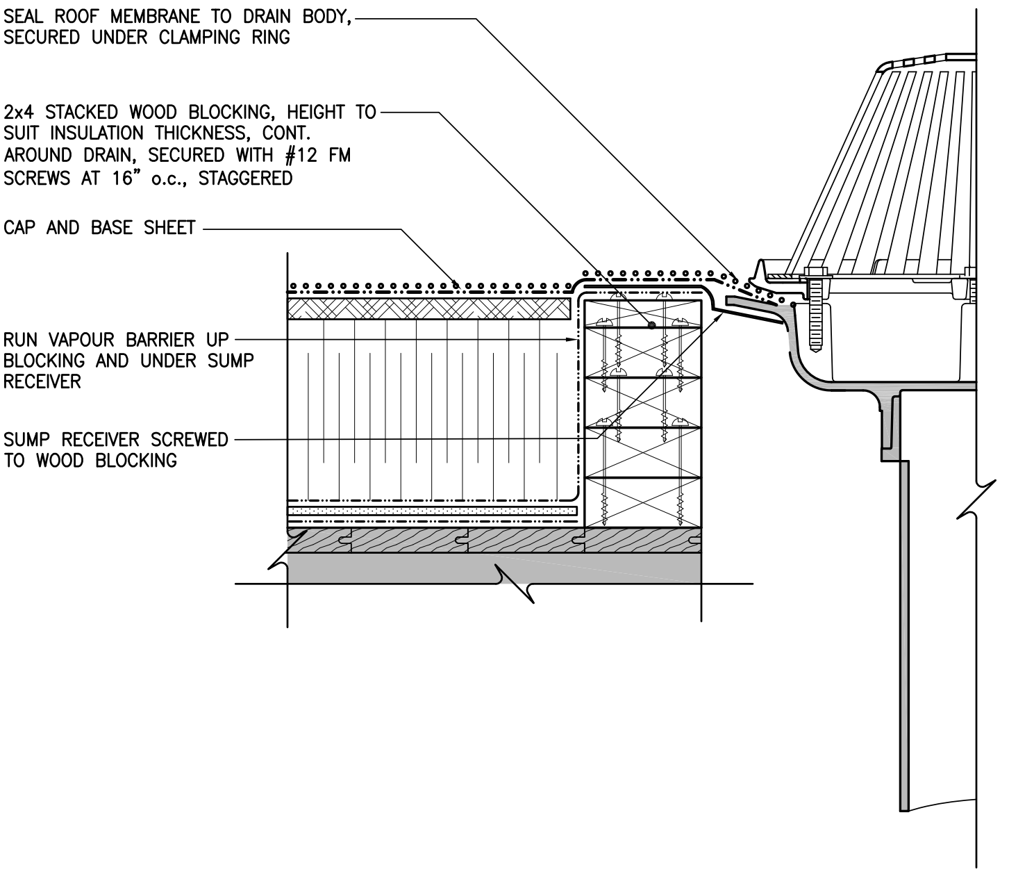
SECTION DETAIL ROOF DRAIN
