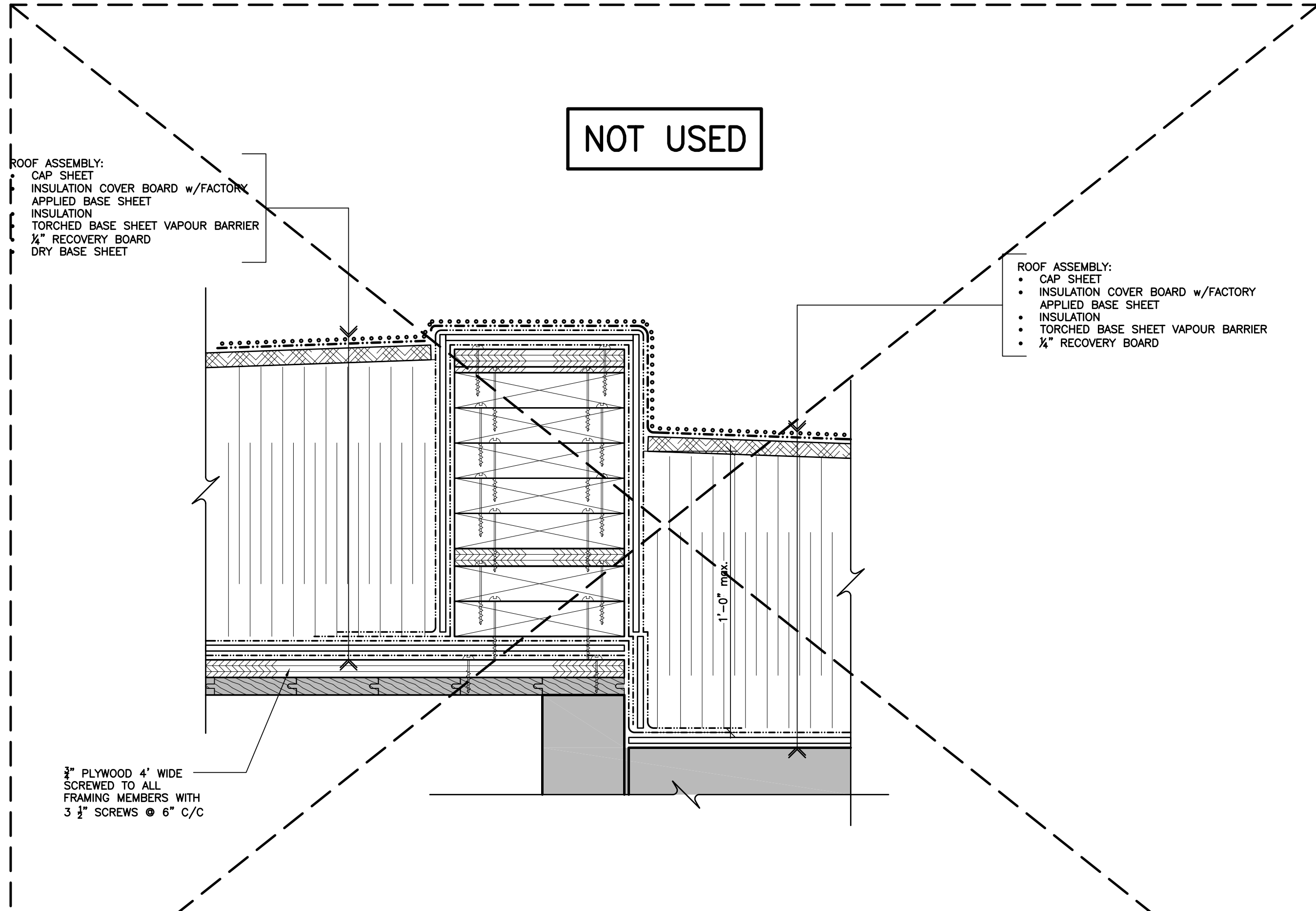
SECTION DETAIL ROOF DIVIDER
