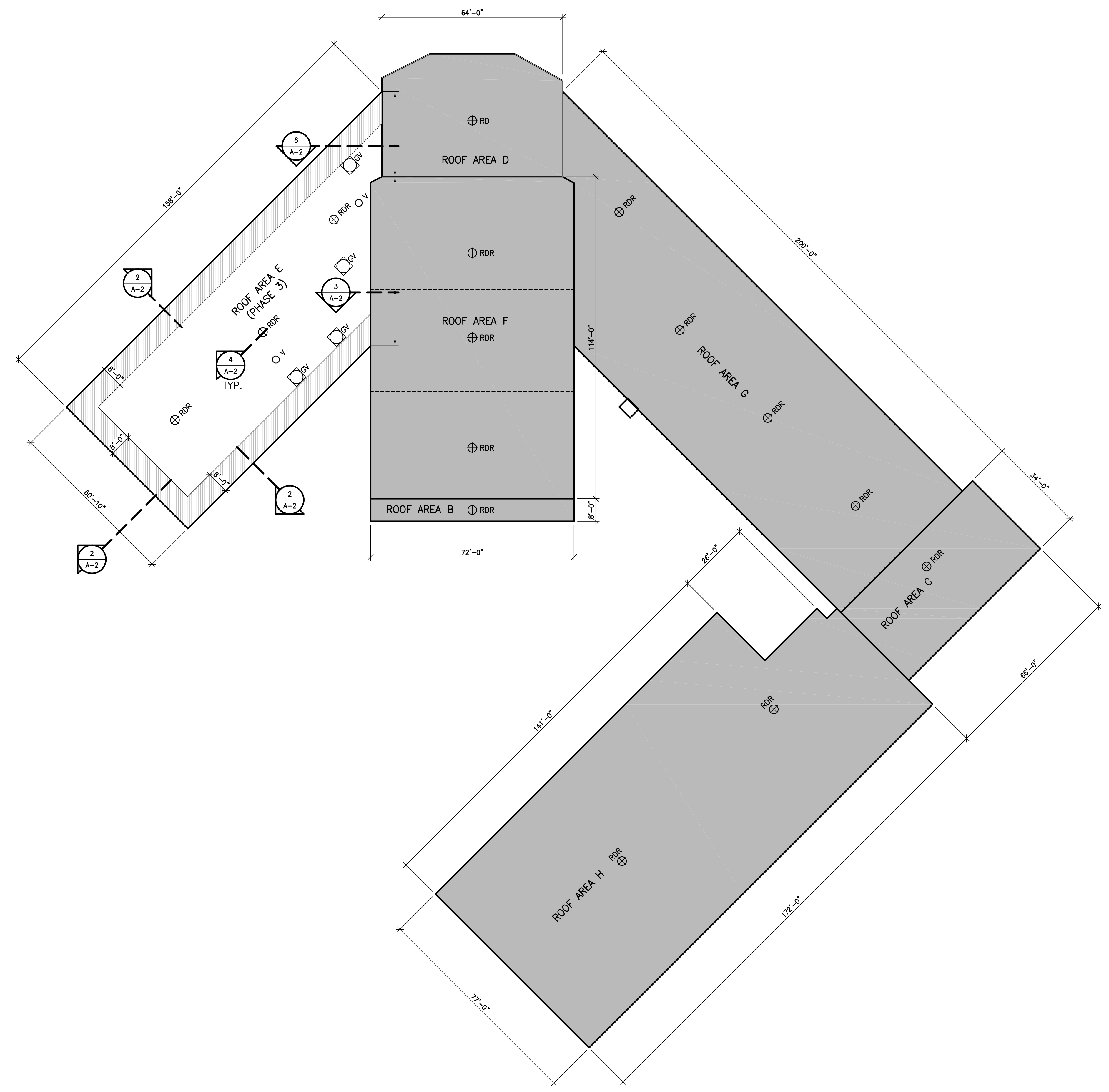
1 A-1 ROOF PLAN SCALE: 1"=20'
