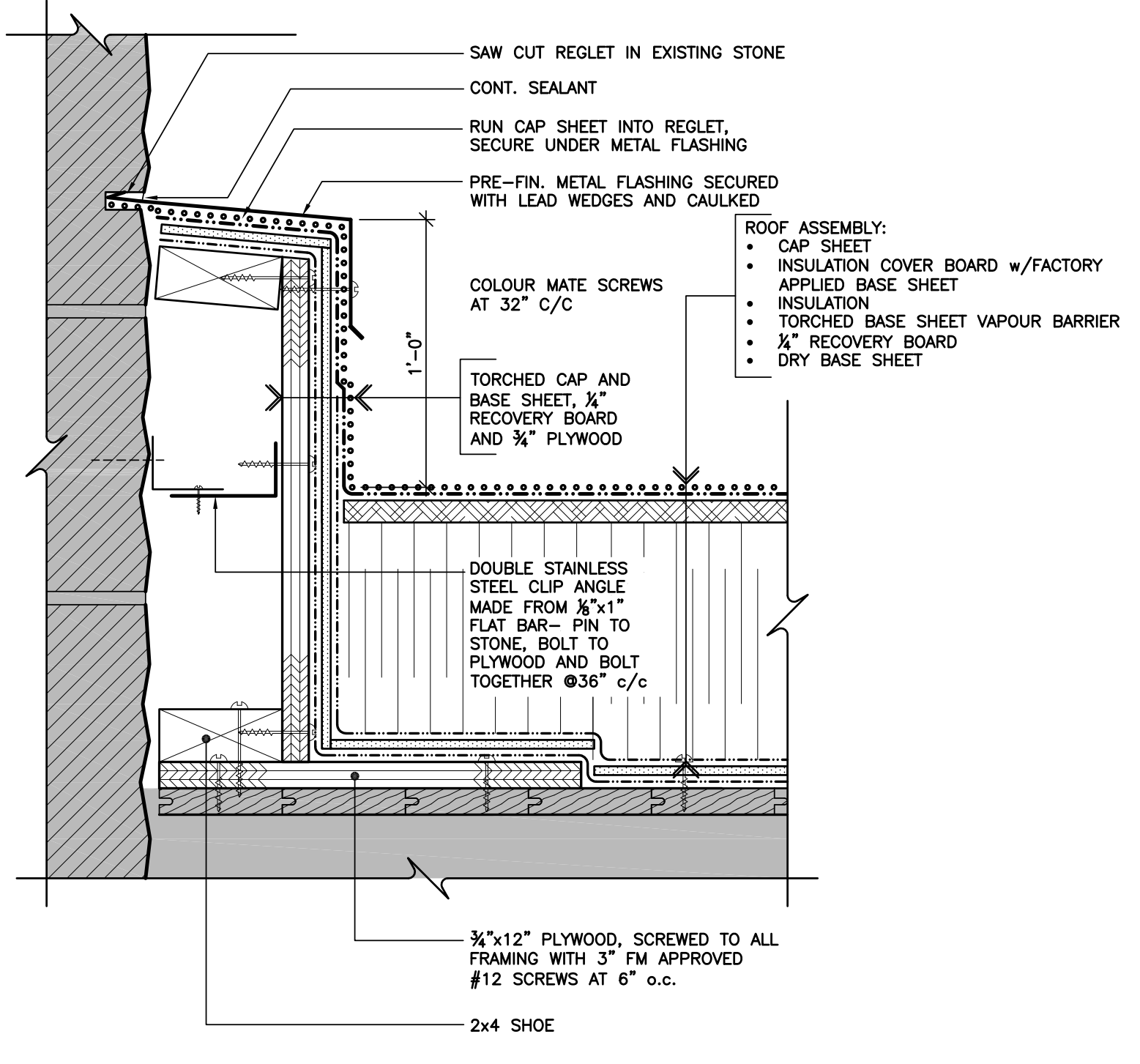
SECTION DETAIL ROOF TO WALL TRANSITION AT STONE WALL
