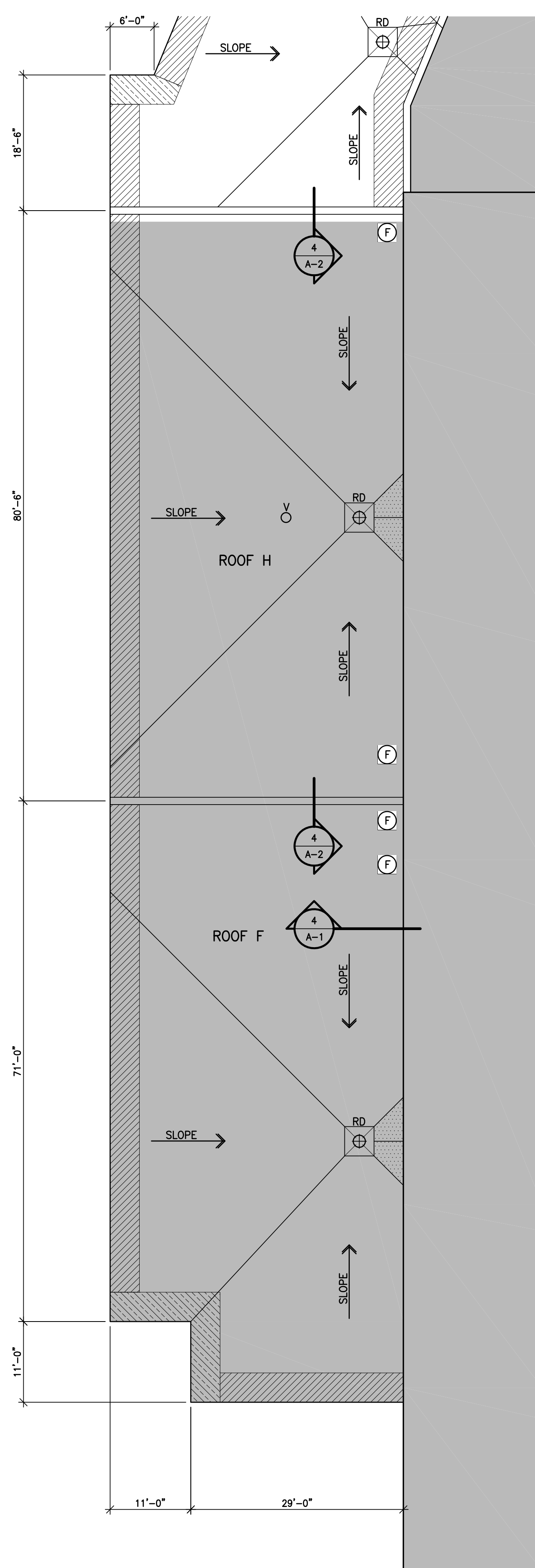
3 A-1 PLAN - ROOF 'H' AND 'F' SCALE: 3/32" = 1'-0"
