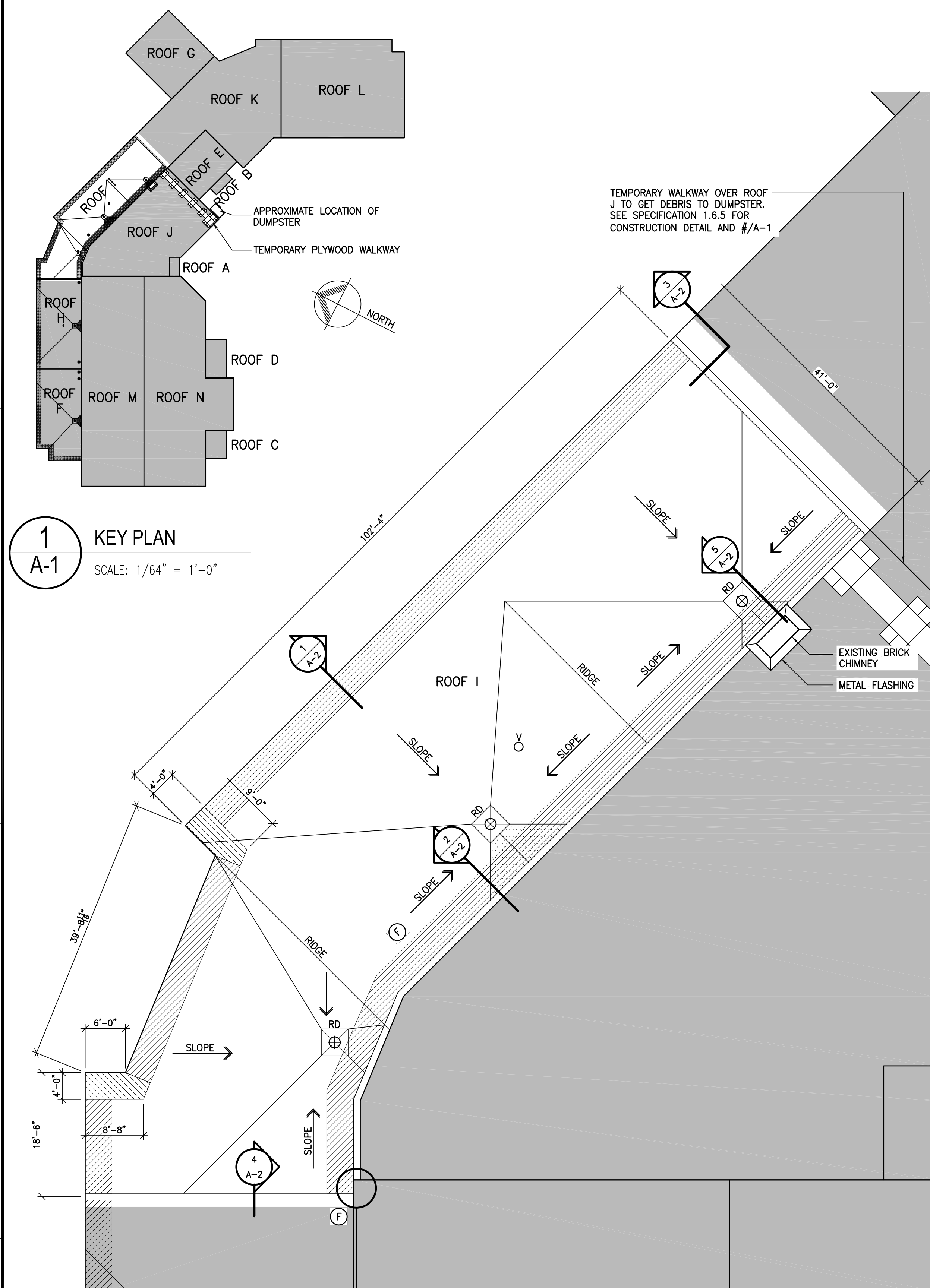
2 A-1 PLAN - ROOF 'I' SCALE: 3/32" = 1'-0"
