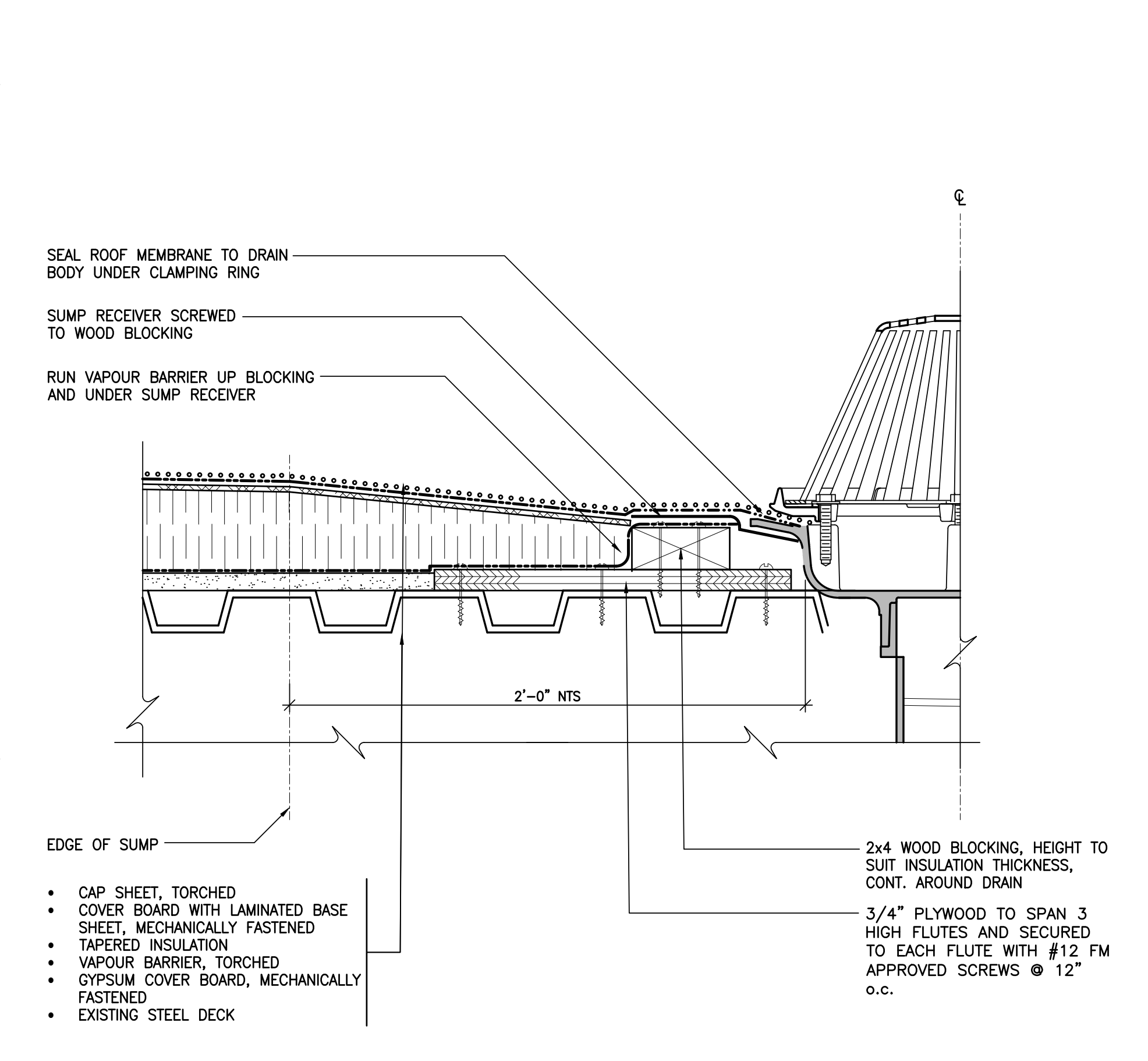
6 A-2 SECTION DETAIL ROOF DRAIN SCALE: 3" = 1'-0"
