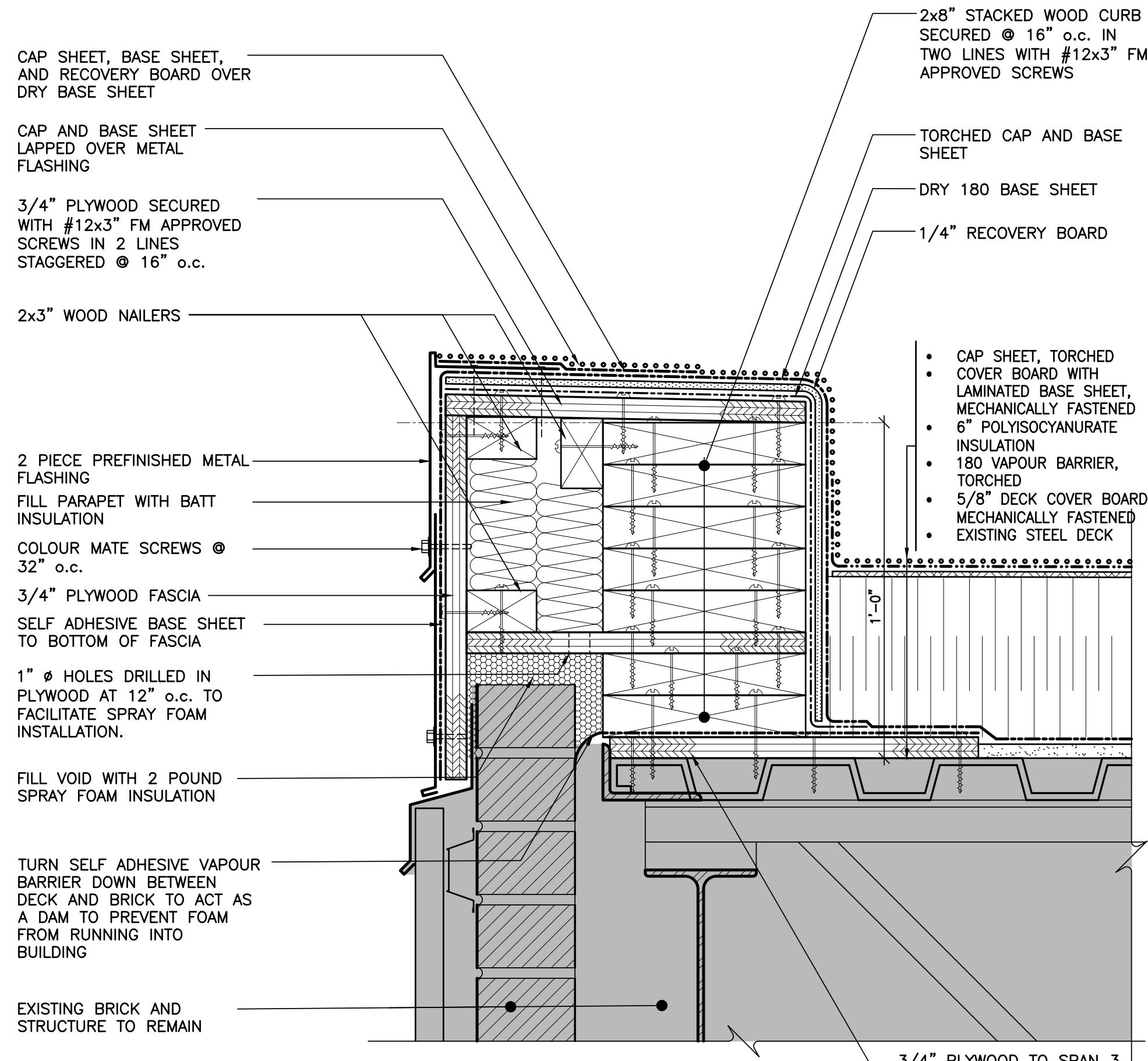
2 A-2 SECTION DETAIL ROOF EDGE AT METAL CLADDING SCALE: 3" = 1'-0"
