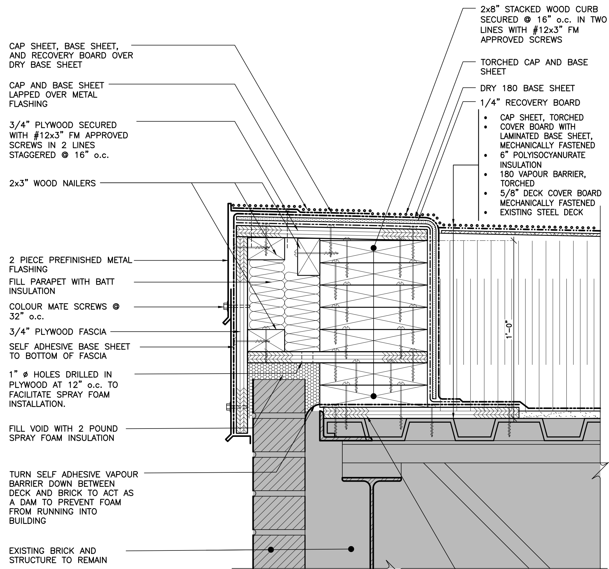
1 A-2 SECTION DETAIL ROOF EDGE AT BRICK SCALE: 3" = 1'-0"
