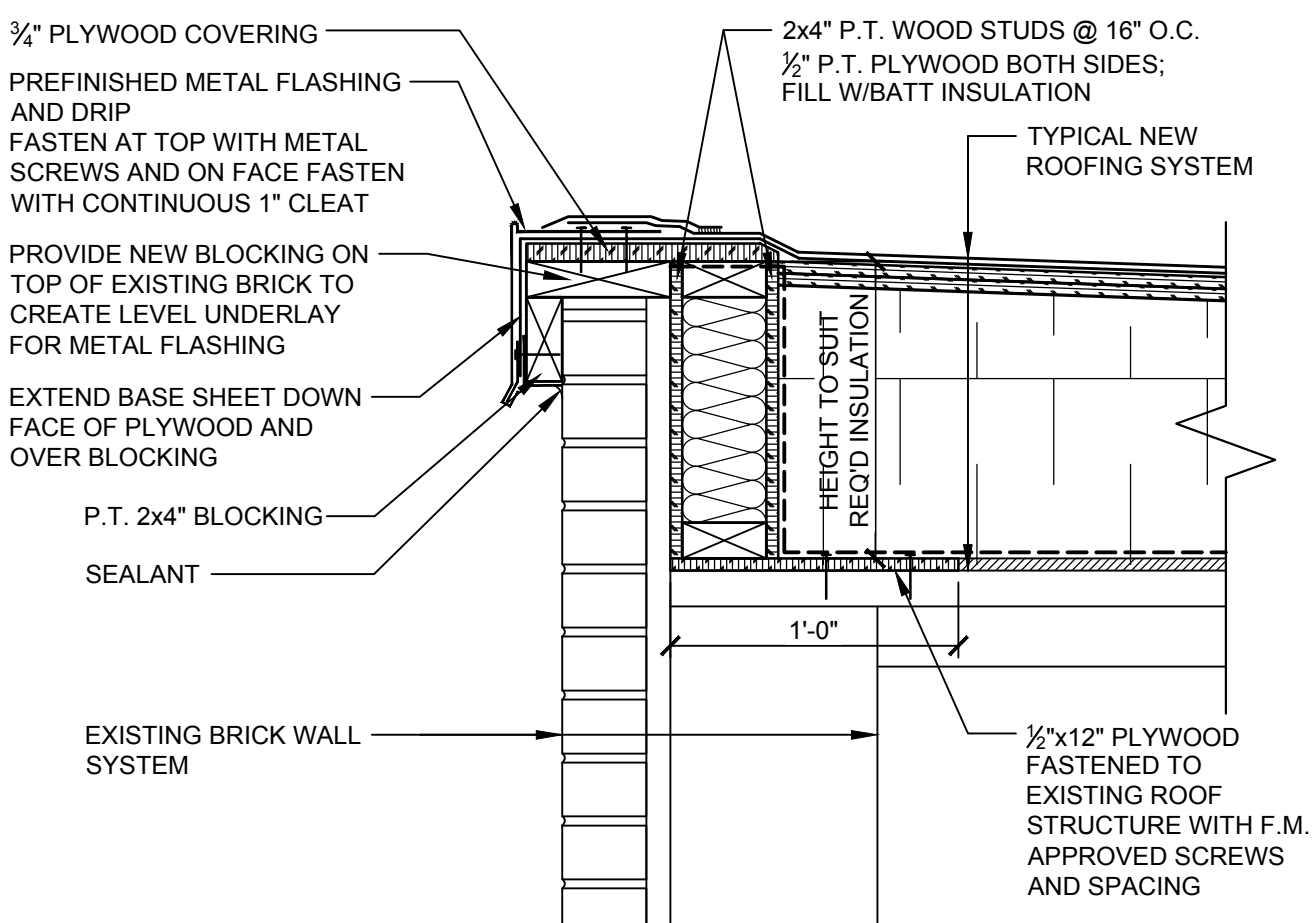
2 PARAPET DETAIL A-101 1-1/2"-1'-0"
