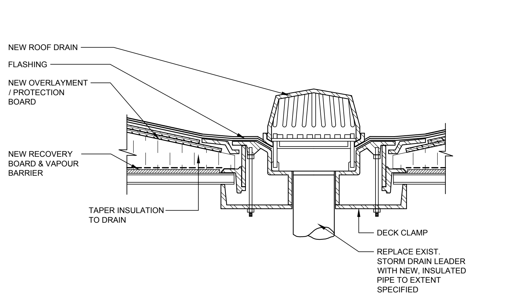
5 ROOF DRAIN DETAIL A-101 1-1/2"-1'-0"
