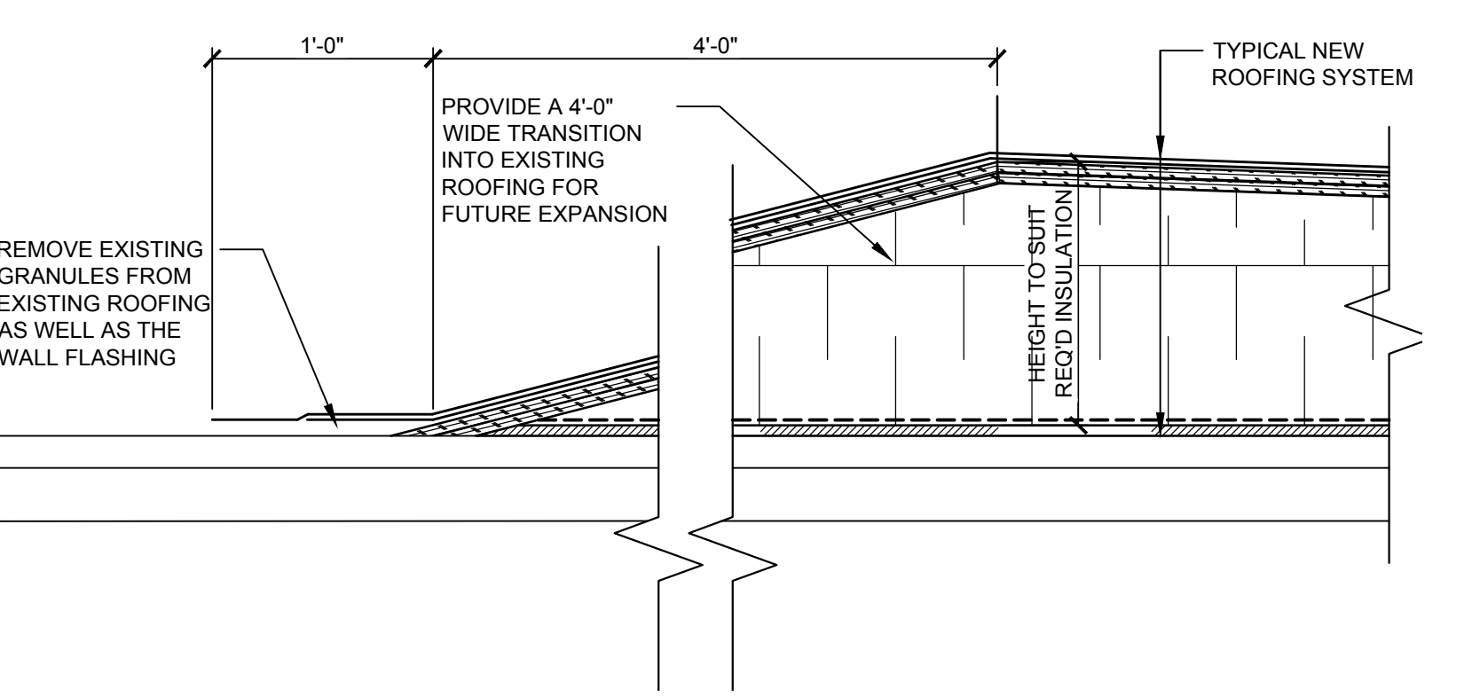
3 ROOF TRANSITION DETAIL A-101 1-1/2"-1'-0"
