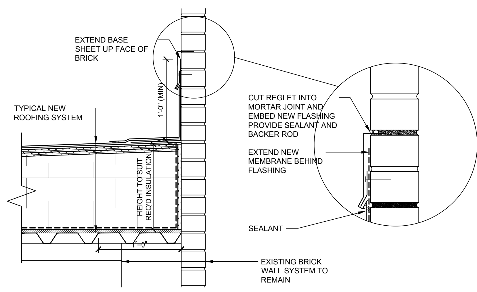
7 CHIMNEY DETAIL A-101 1-1/2"-1'-0"
