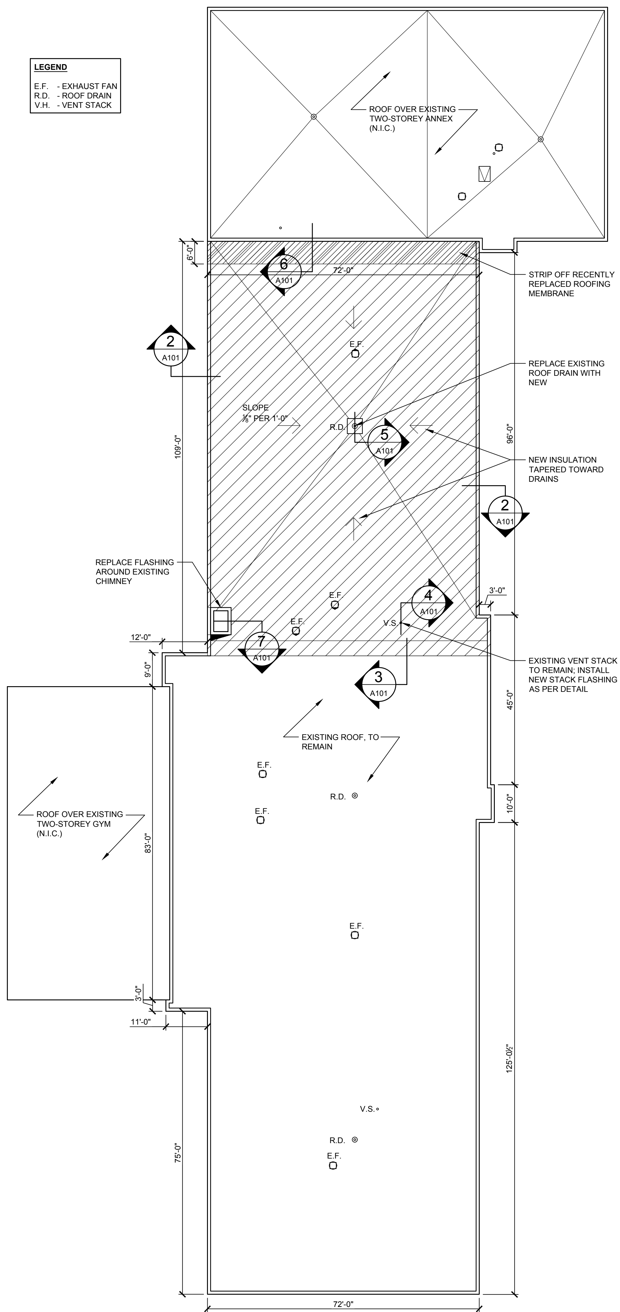
1 OVERALL ROOF PLAN A-101 1/16"-1'-0"
