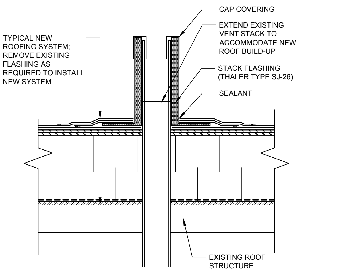
4 VENT STACK DETAIL A-101 1-1/2"-1'-0"
