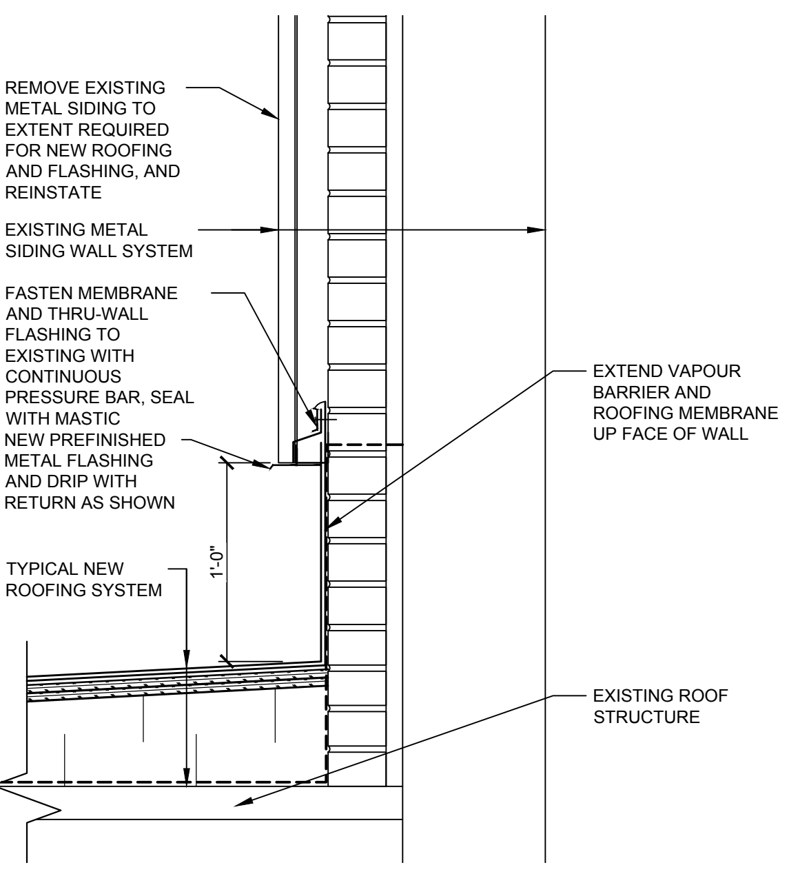
6 EXISTING WALL DETAIL A-101 1-1/2"-1'-0"
