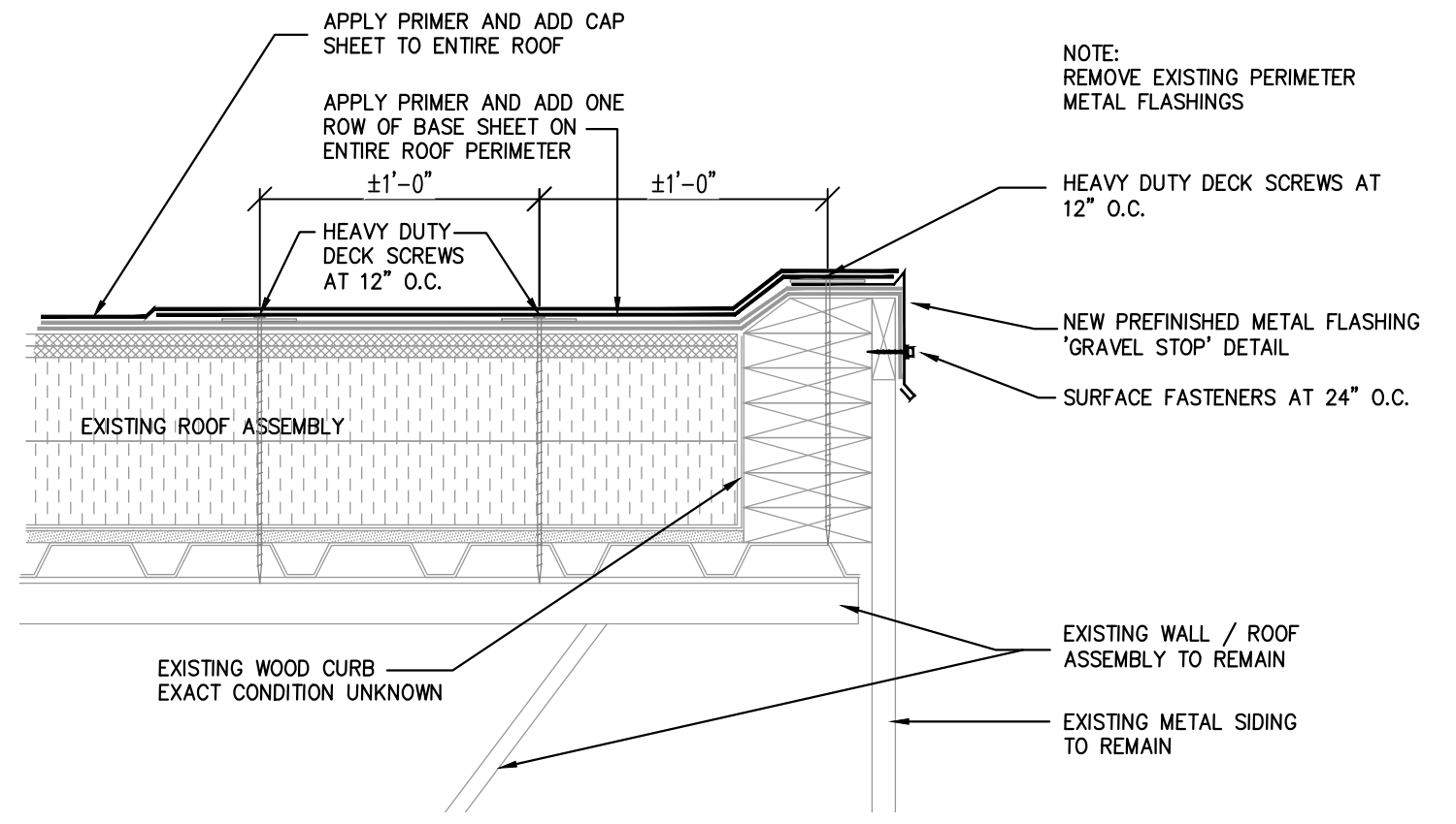
1 1/2"=1'-0" 1 TYPICAL PARAPET DETAIL A-301
