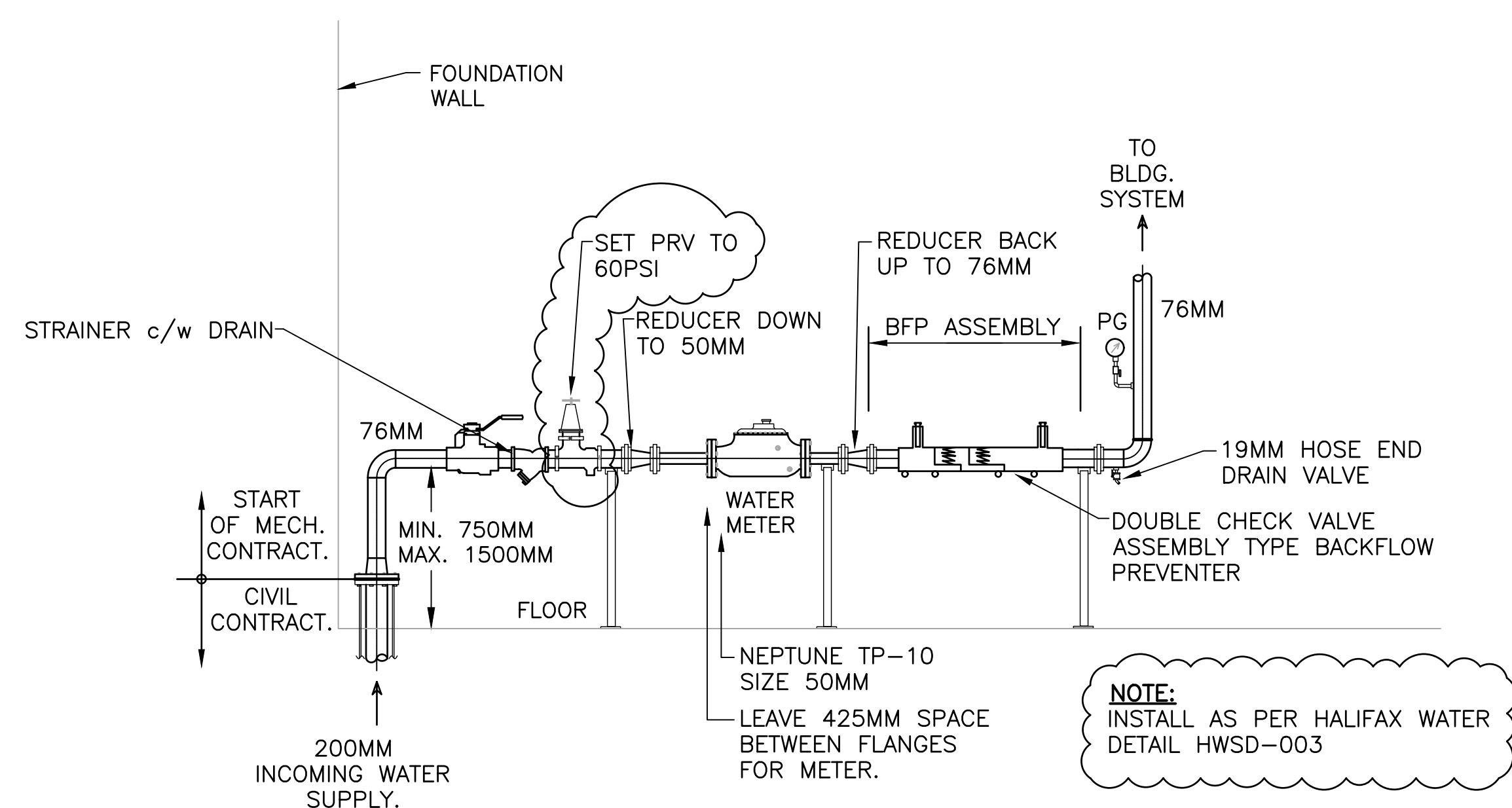
2 DETAIL—WATER METER ASSEMBLY NTS
