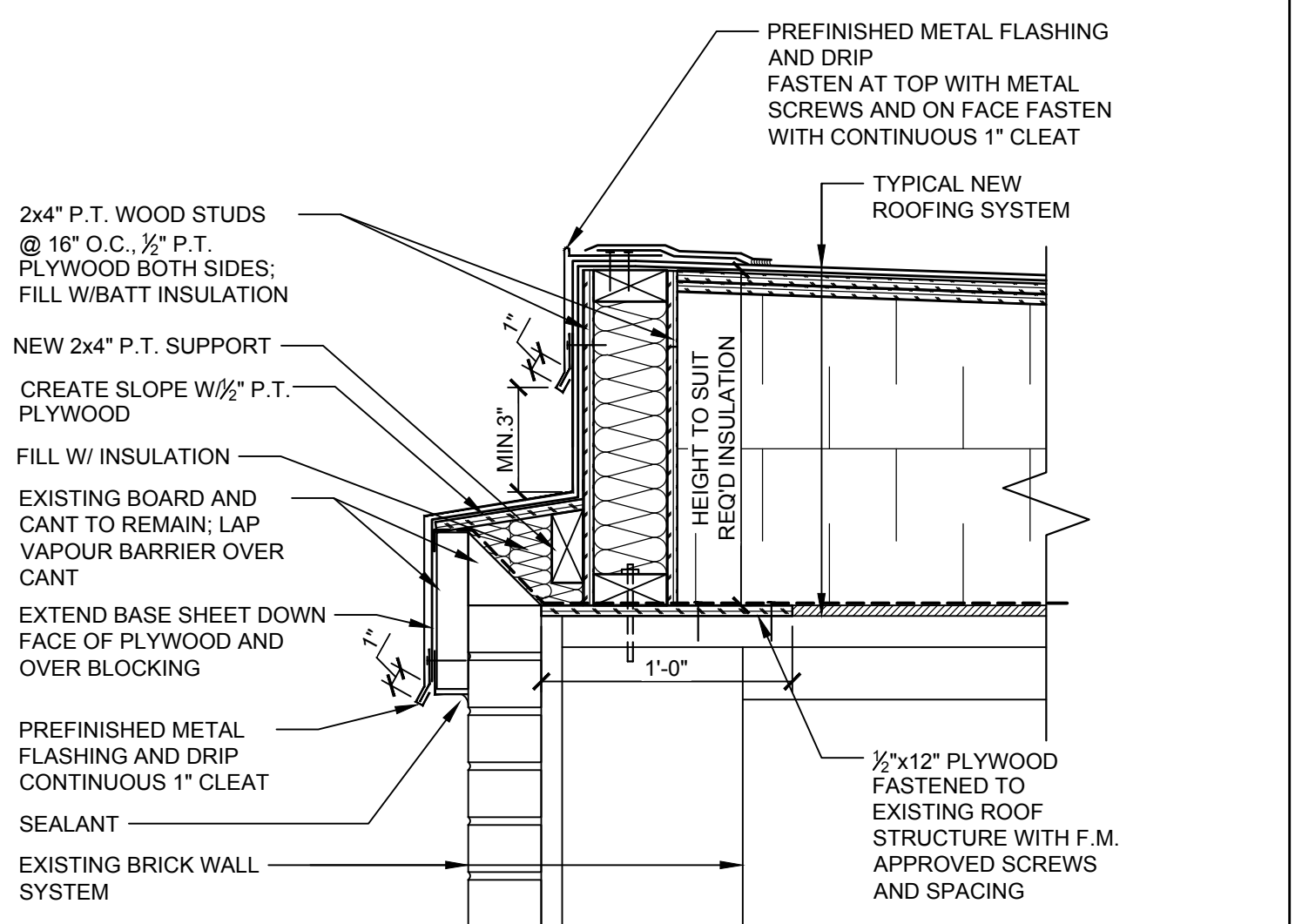
2 PARAPET DETAIL A-101 1-1/2"=1'-0"
