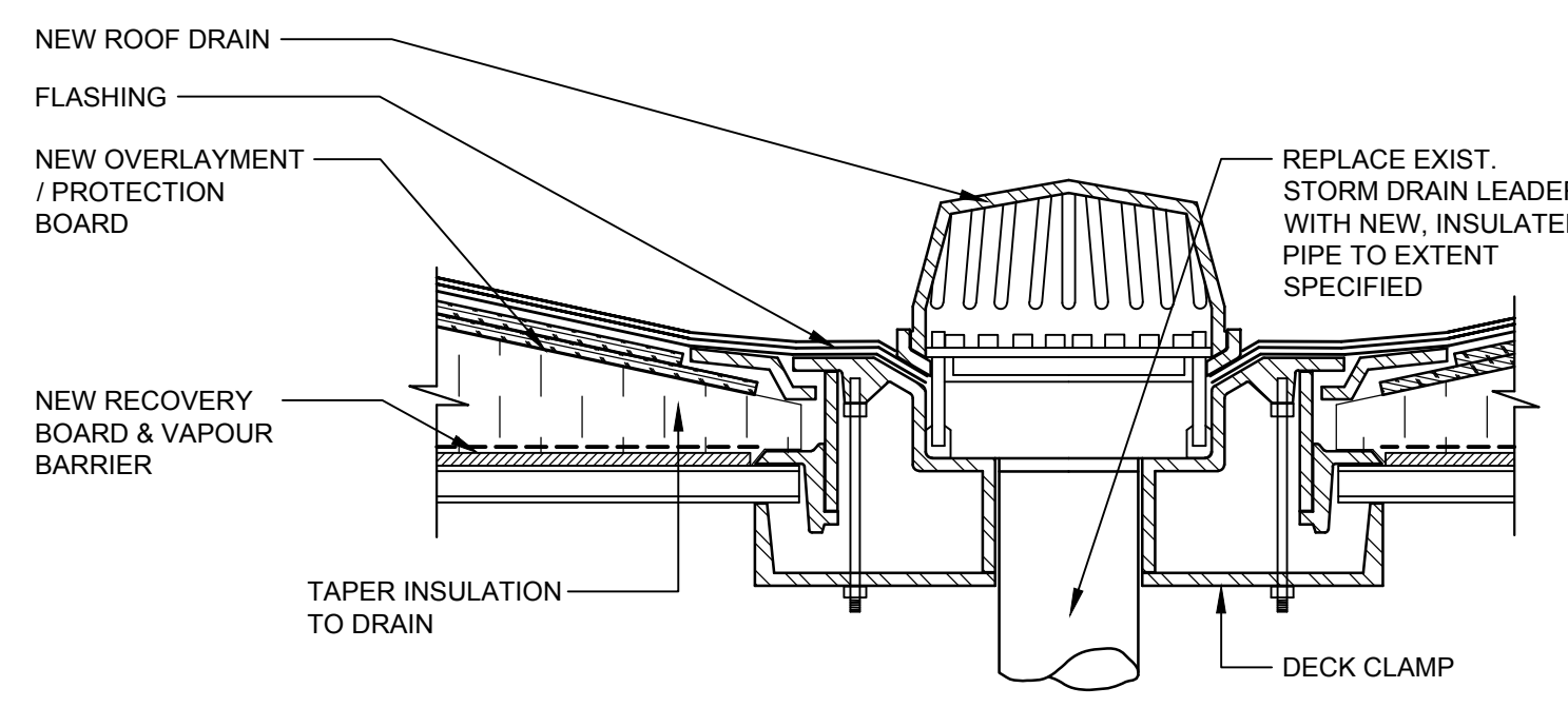
6 ROOF DRAIN DETAIL A-101 1-1/2"=1'-0"
