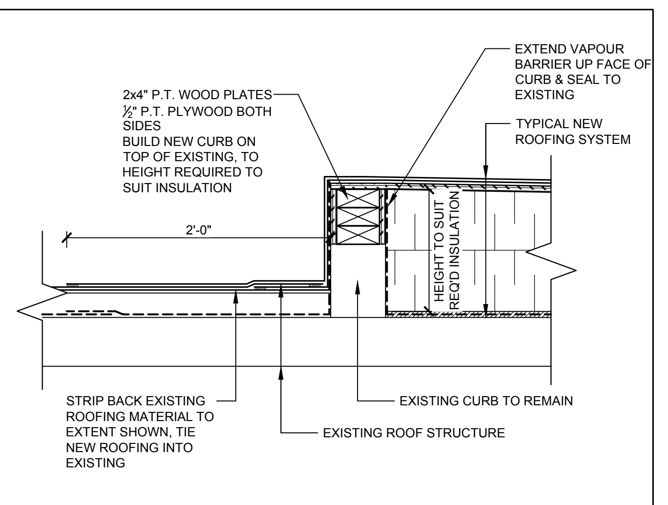
3 ROOF TRANSITION DETAIL A-101 1-1/2"=1'-0"
