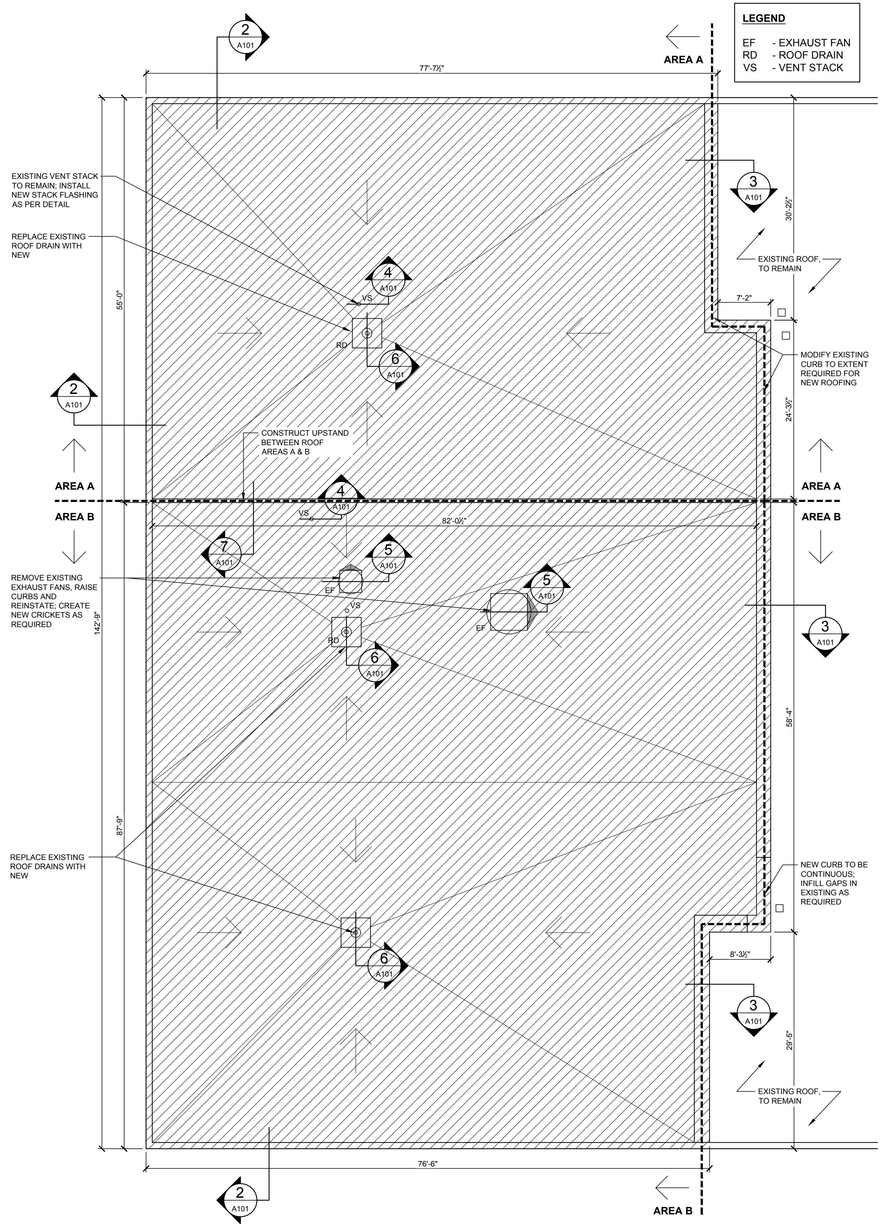
1 PARTIAL ROOF PLAN A-101 1/8"=1'-0"
