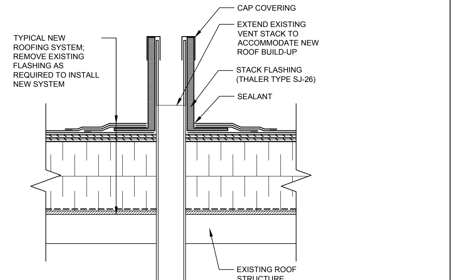
4 VENT STACK DETAIL A-101 1-1/2"=1'-0"
