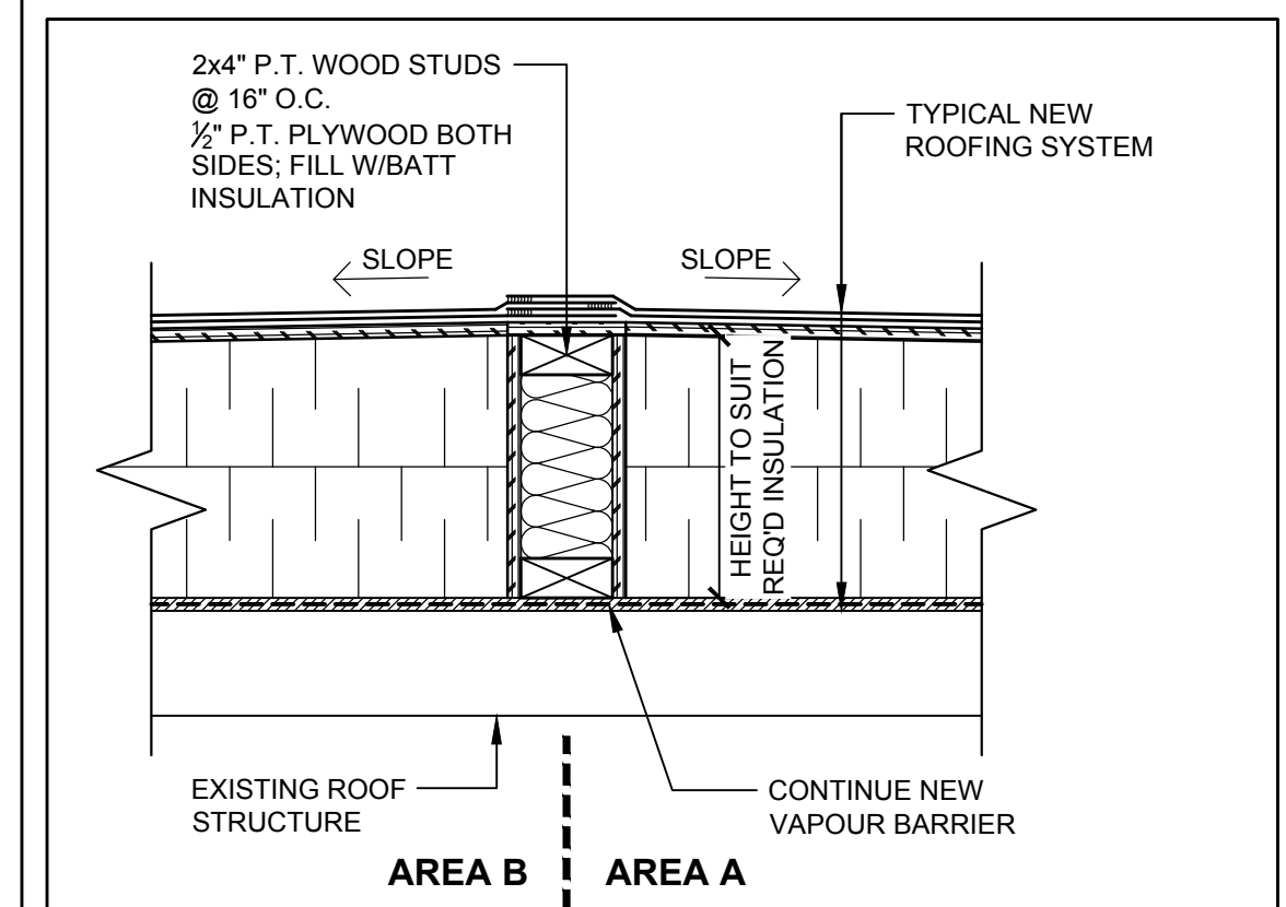
7 ROOF TRANSITION DETAIL A-101 1-1/2"=1'-0"
