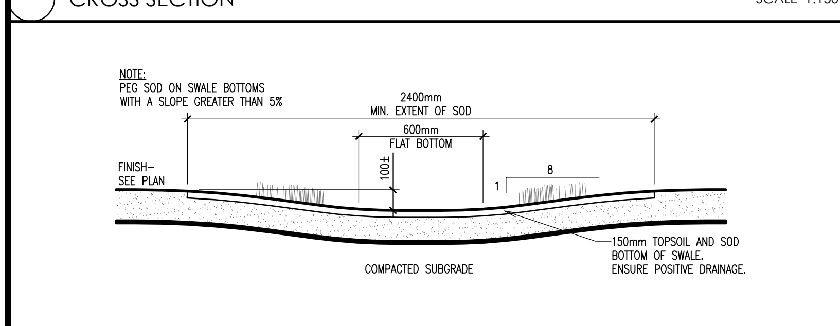
4 SWALE SCALE 1:20
