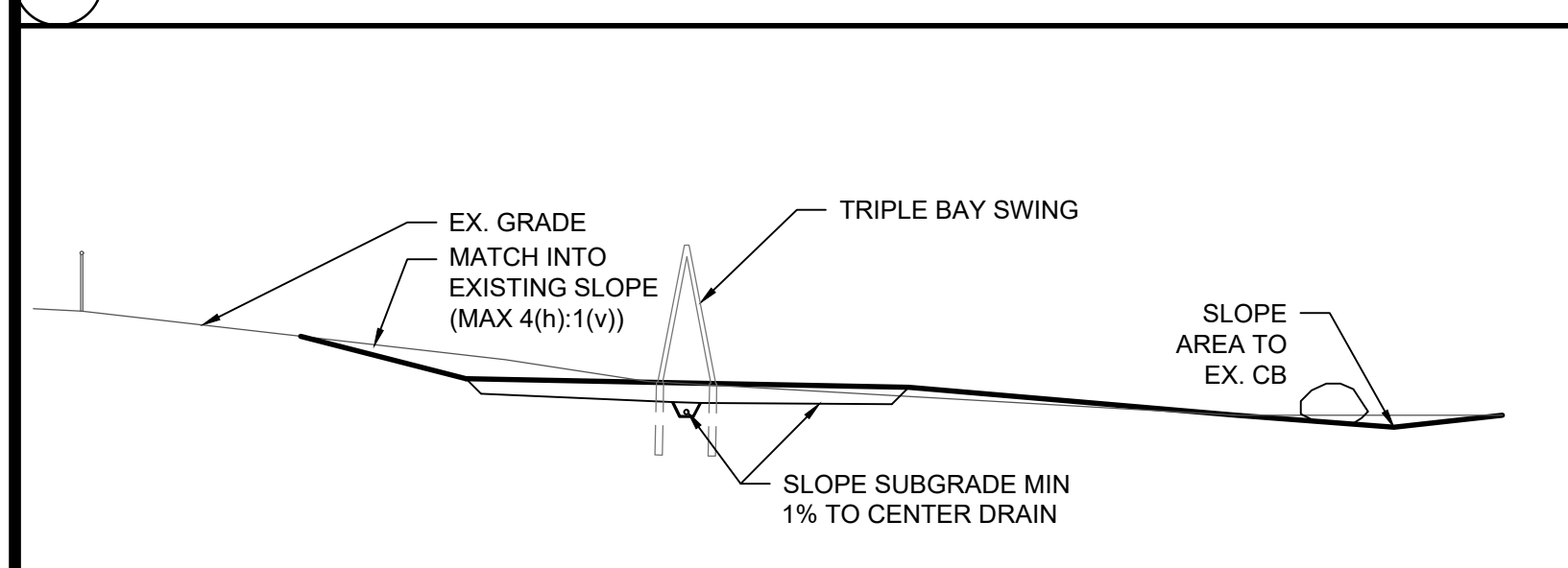
3 CROSS SECTION SCALE 1:150
