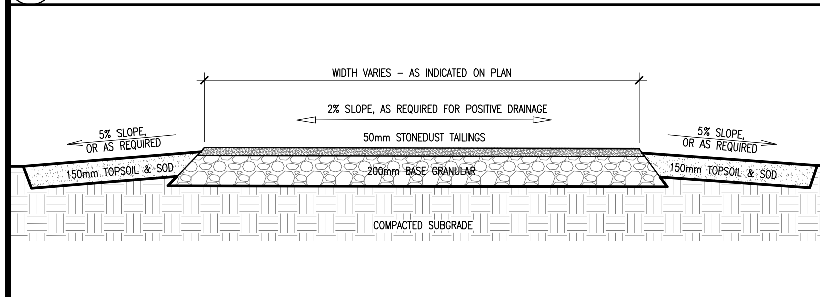
2 STONEDUST SURFACING SCALE 1:25
