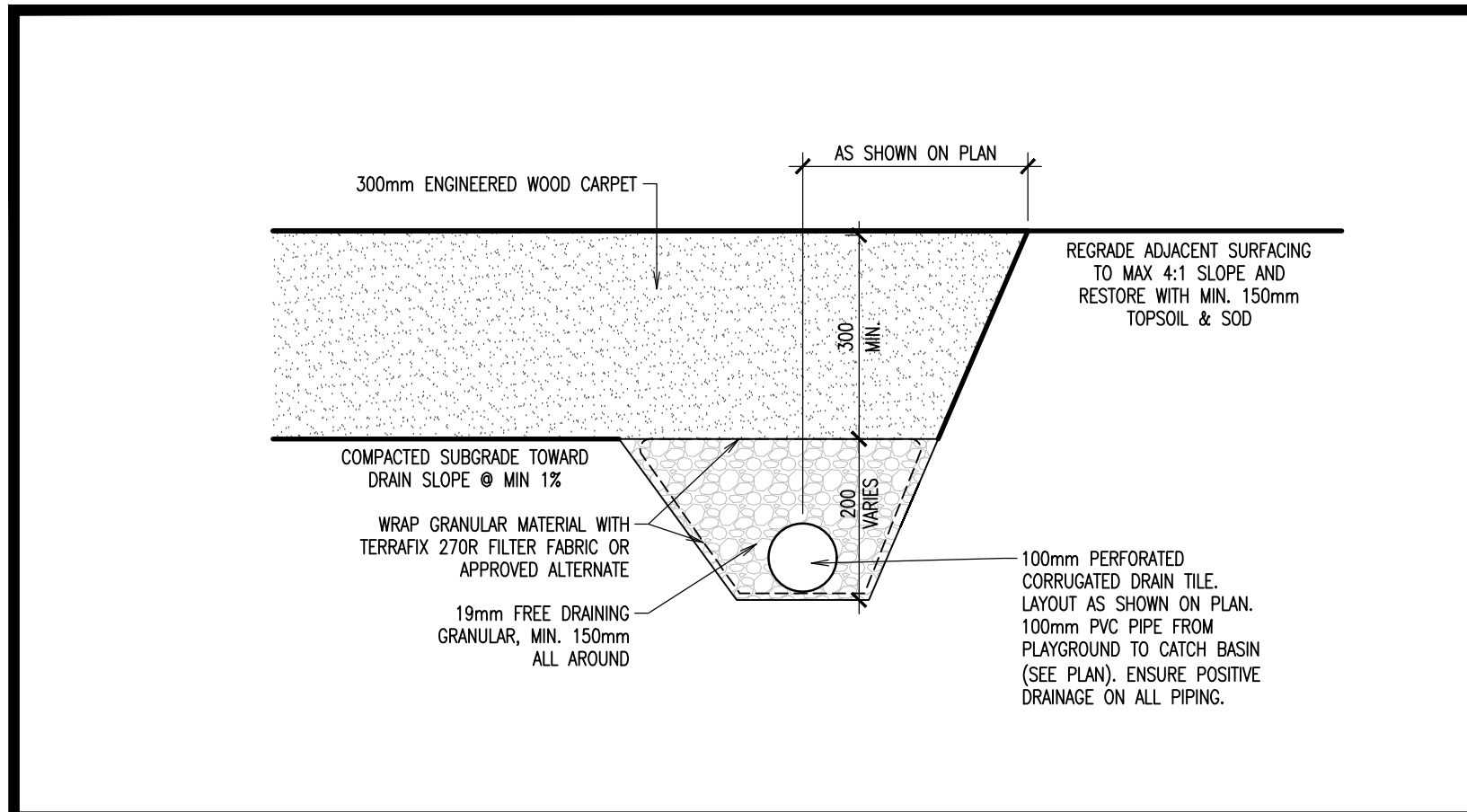
1 PLAYGROUND SURFACING SCALE 1:10
