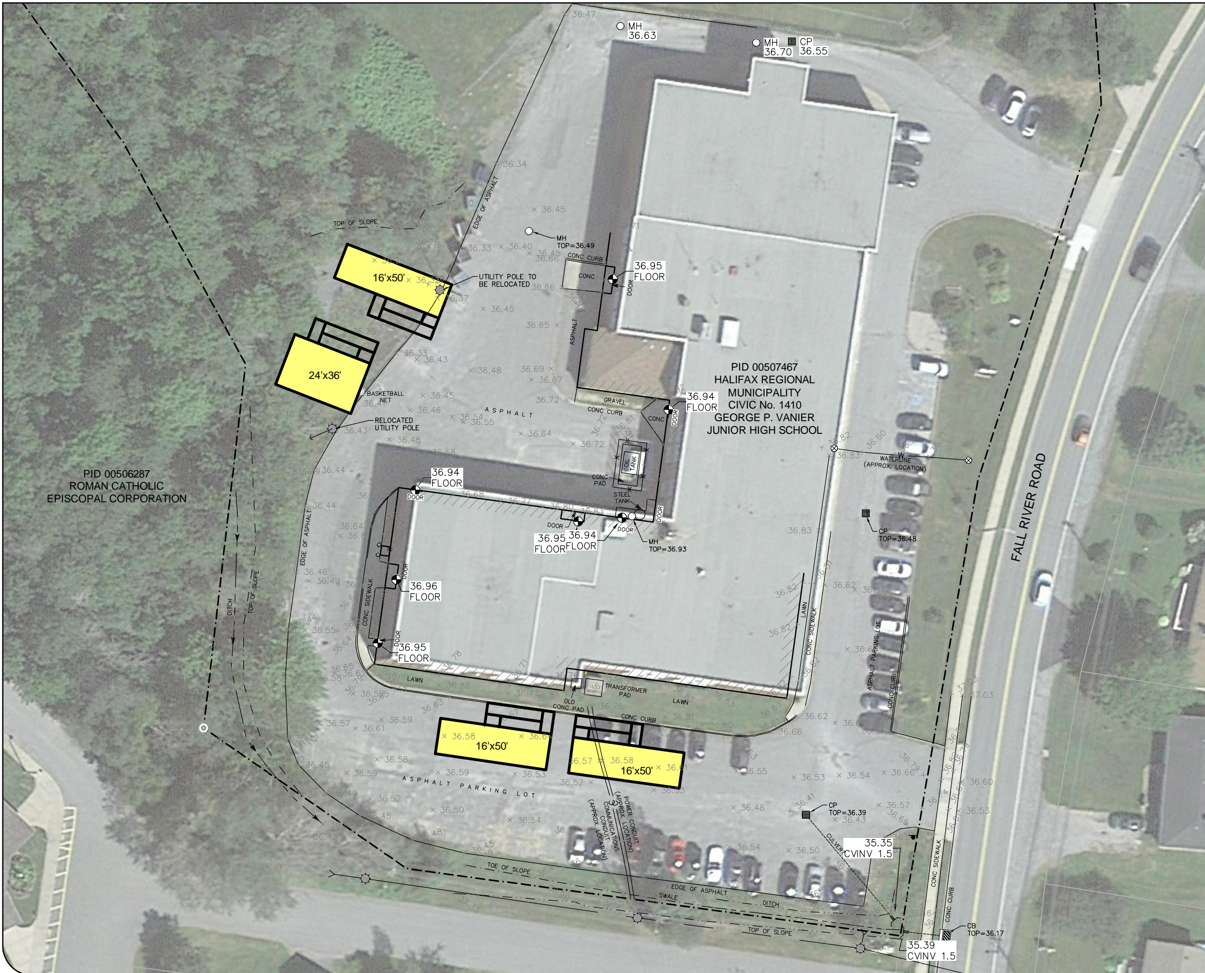
PROPOSED LAYOUT FIGURE 1
