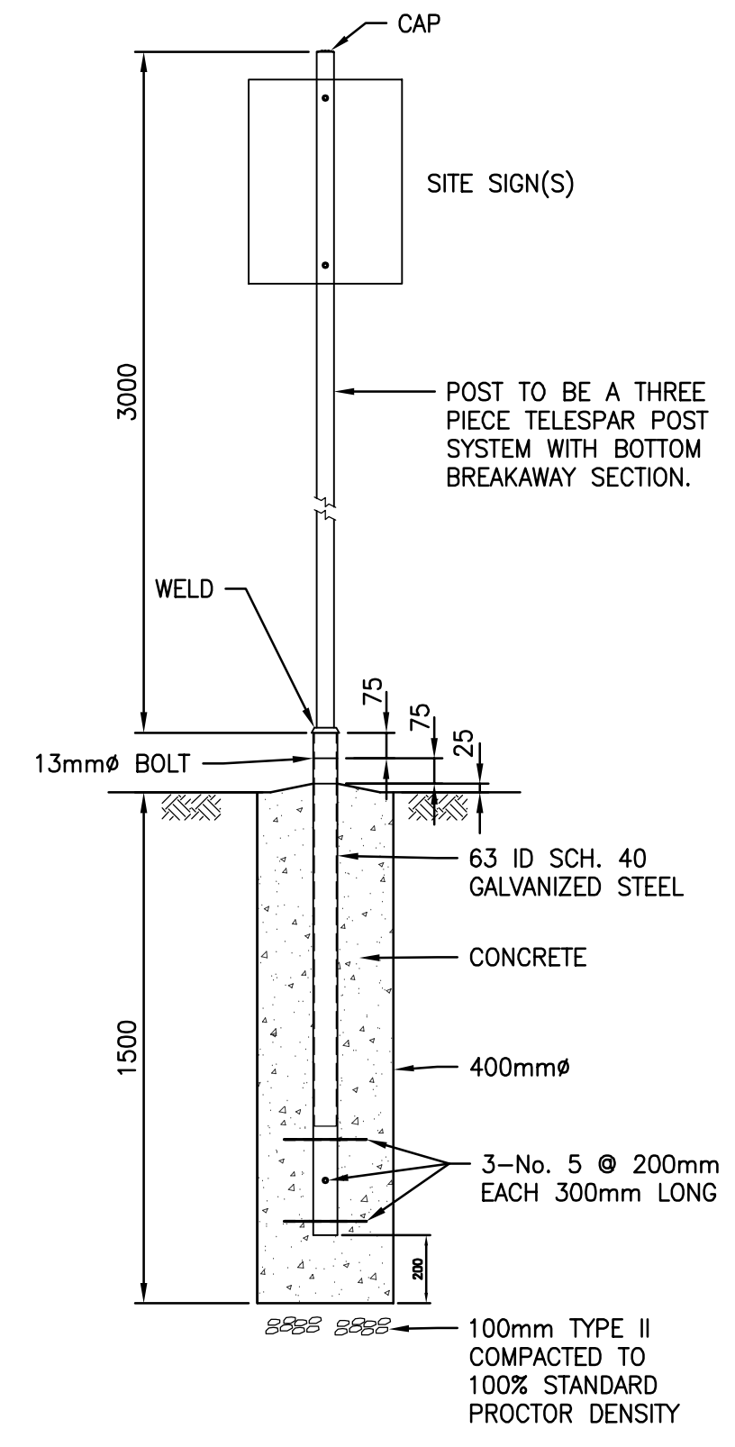
PARKING SPOT SIGN DETAIL N.T.S.
