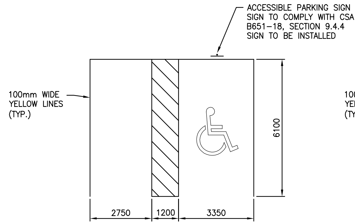
ACCESSIBLE PARKING STALL DETAILS N.T.S.
