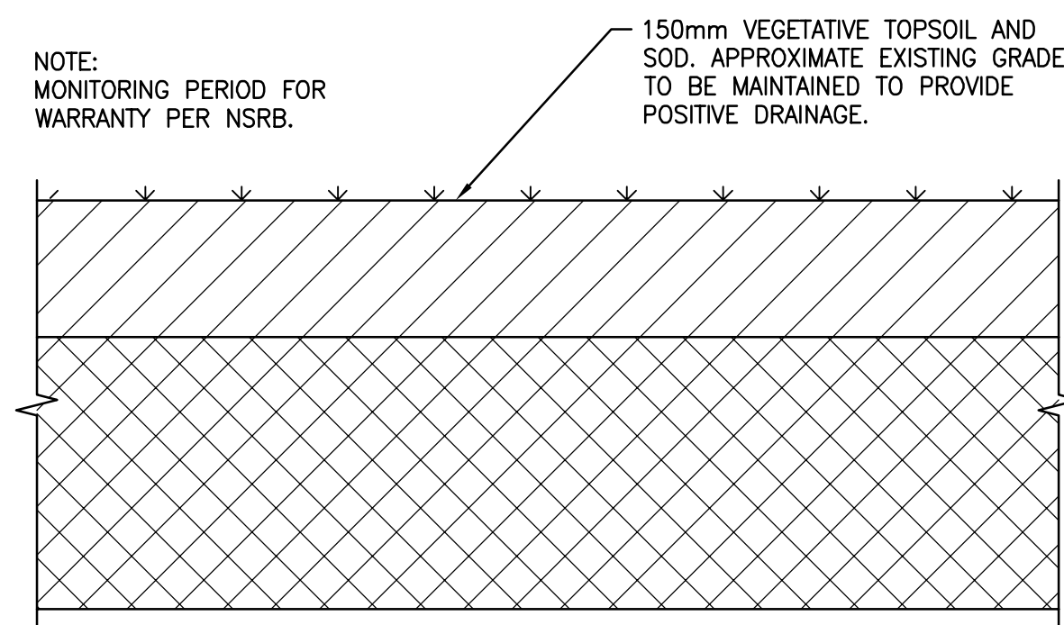
TYPICAL TOPSOIL AND SOD REINSTATEMENT DETAIL N.T.S.
