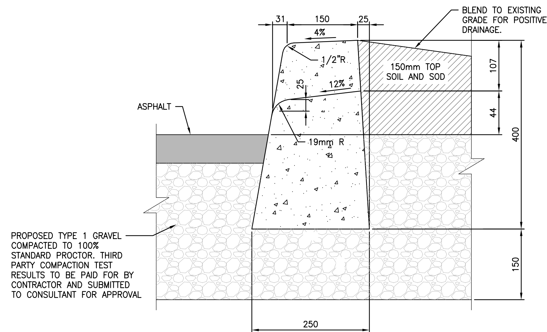
TYPICAL CONCRETE CURB DETAIL N.T.S.
