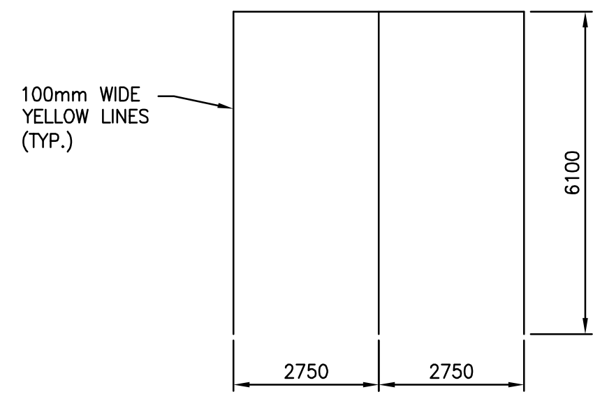
PARKING STALL DETAILS N.T.S.
