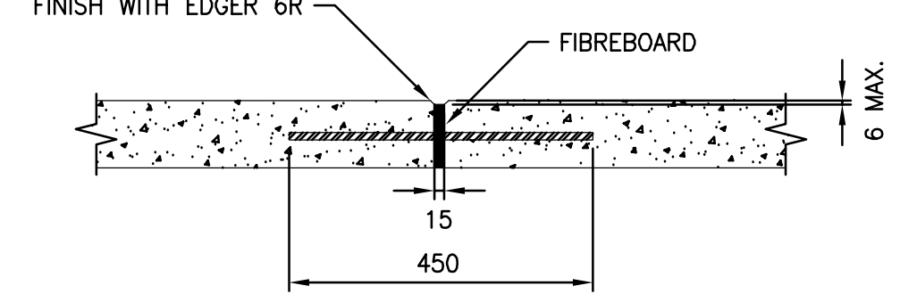
EXPANSION JOINT 1:10
