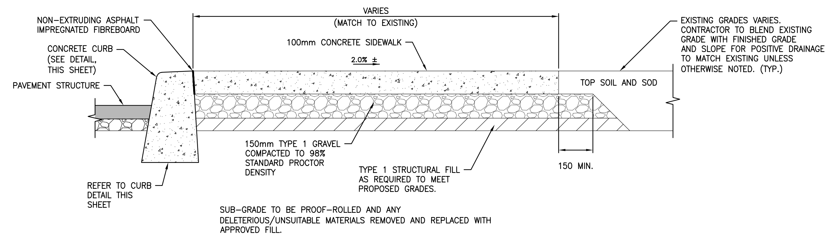
SIDEWALK CROSS-SECTION 1:10
