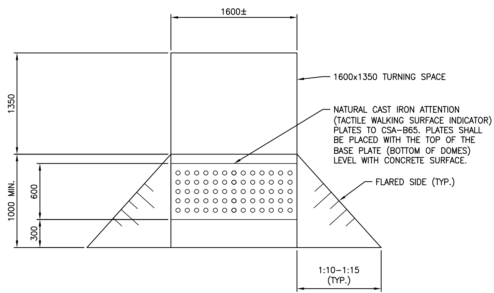
PEDEDTRIAN CURB RAMP/TACTILE WALKING SURFACE INDICATOR (TWSI) N.T.S.
